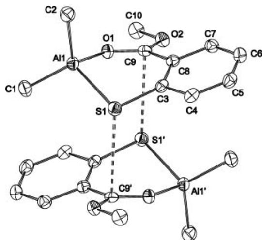
Figure 1. Molecular structure of 1 with thermal ellipsoids drawn at the 40% probability; hydrogen atoms are omitted for clarity.
