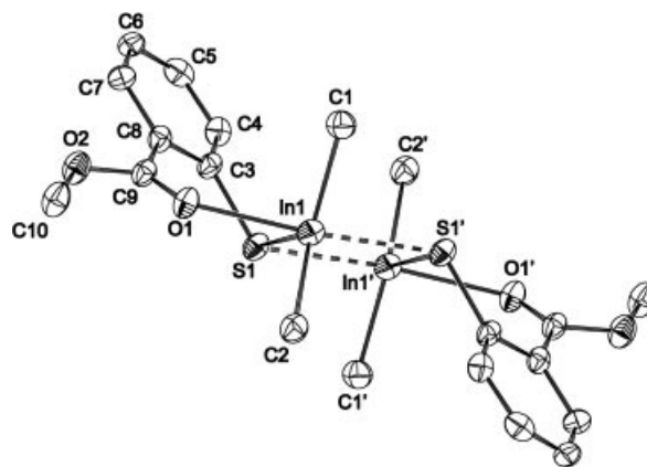
Figure 2. Molecular structure of 2 with thermal ellipsoids drawn at the 40% probability; hydrogen atoms are omitted for clarity.
